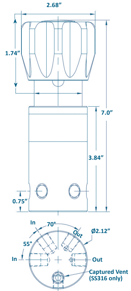
Figure 2: Series 3000 SS316 dimensions
