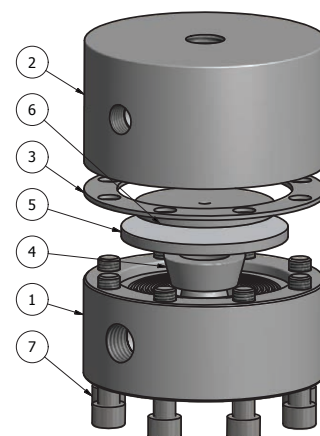
Figure A: Exploded View Mity Mite Replacement Regulator
