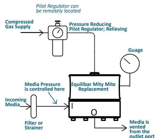
Fig. 1 Mity Mite Replacement Setup
