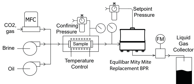
Fig. 2 Core Analysis Pressure Control
