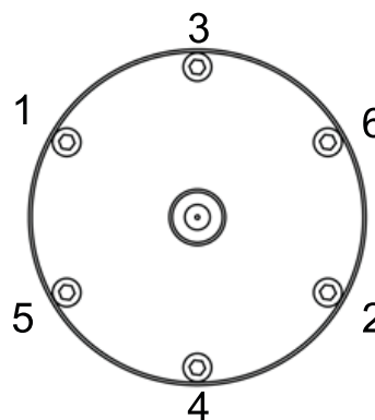
Figure B: Sample Torque Pattern Larger sizes will have more bolts
