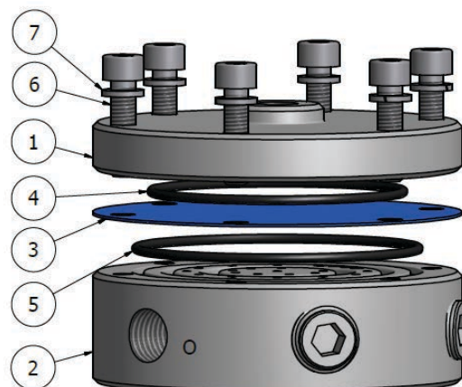
Figure A: Exploded View GS Series
