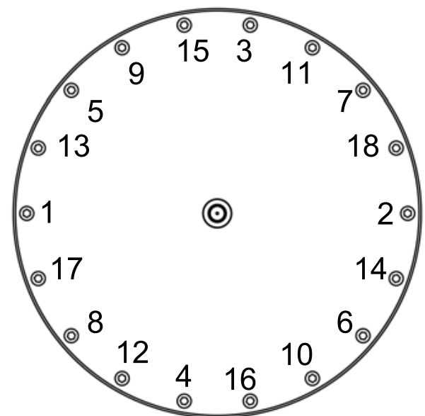
Figure B: Sample Torque Pattern
