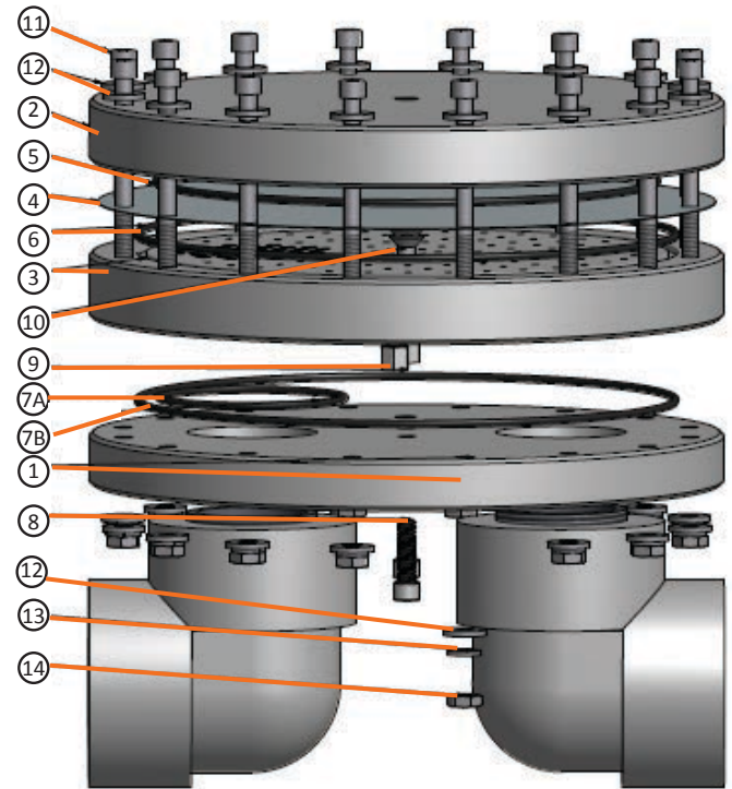
Figure A: Exploded View - Equilibar BD
