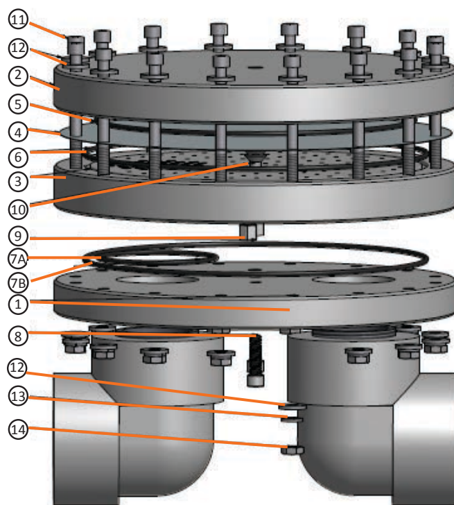
Figure A: Exploded View - Equilibar BD
